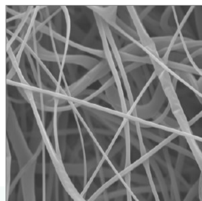
FilterPON: electron microscope photograph
